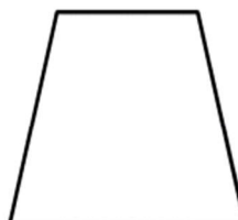
Trapezoid
