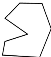
Irregular Octagon
