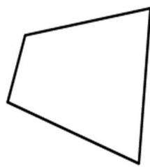
Irregular Quadrilateral
