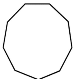
Regular Nonagon
