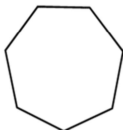
Regular Heptagon
