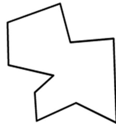
Irregular Decagon
