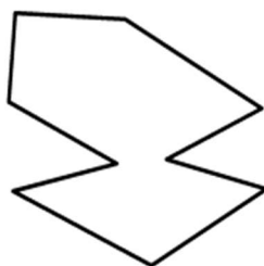
Irregular Nonagon
