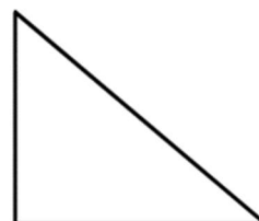
Right Triangle
