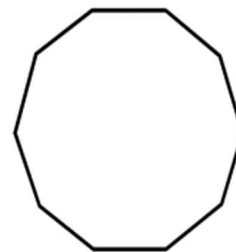
Regular Decagon
