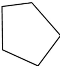
Irregular Pentagon
