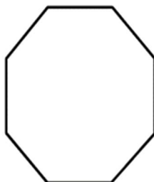
Regular Octagon
