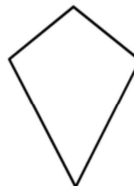
Kite
