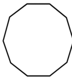
Regular Decagon
