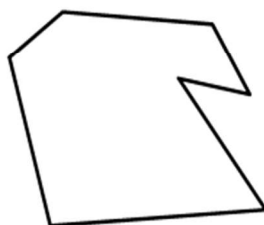
Irregular Heptagon
