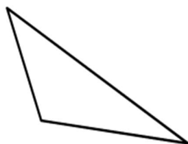
Irregular Triangle
