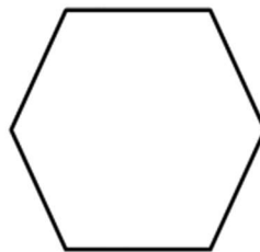
Regular Hexagon
