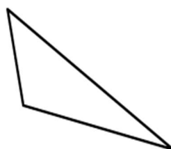
Scalene Triangle
