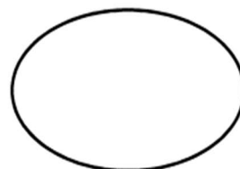
Ellipse
