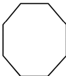
Regular Octagon
